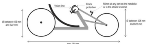
Figure 2. Handbike
