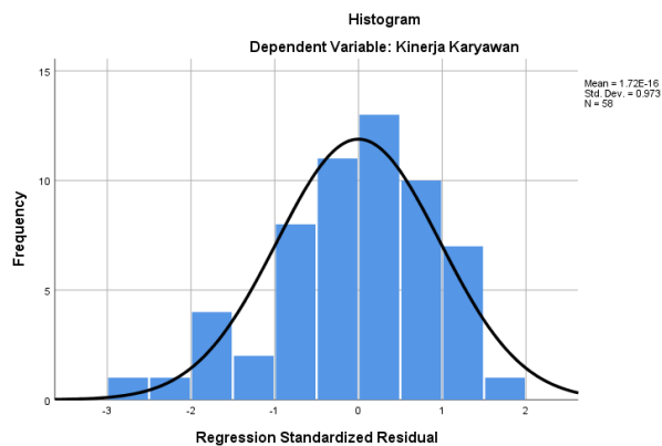
Gambar 3. Uji NormalitasHistogram
