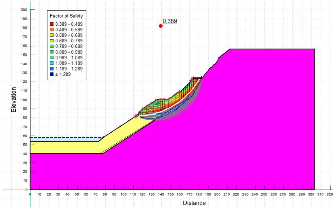
Figure 9. Unreinforced slope
