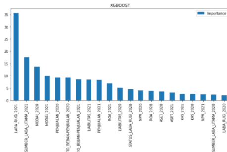
Gambar 8. Features Important
