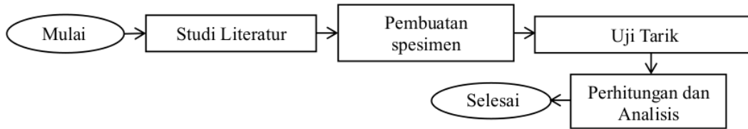
Gambar 1. Flowchart
