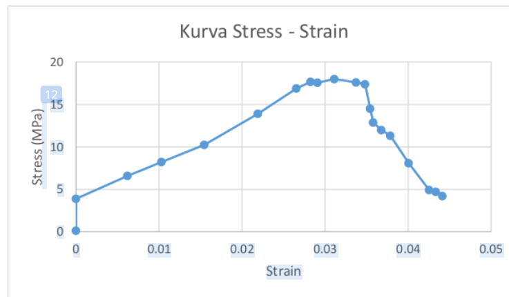
Gambar 3. Kurva stress-strain komposit sabut kelapa
