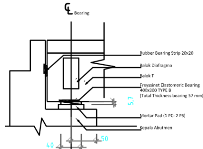
Gambar 8. Detail elastomeric bearing
