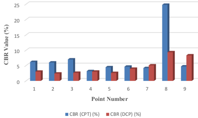
Fig. 4. Graph of Ratio between CBR_{(CPT)} and CBR_{(DCP)}
