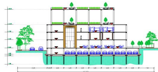
Gambar 18. Gambar tampak Roofgarden
